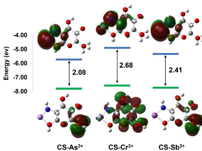
Figure 4 Energy diagram of HOMO and LUMO orbitals (in eV) of CS-trivalent metal cation complexes.
