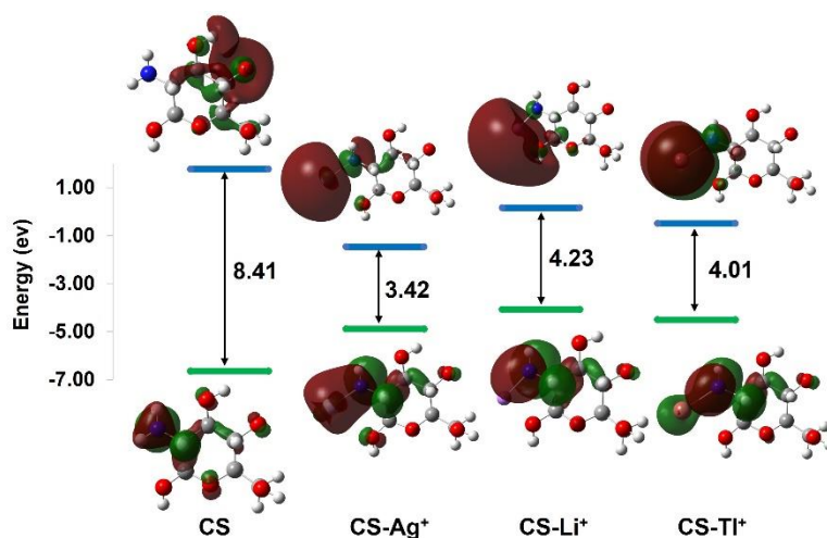
Figure 2 Energy diagram of HOMO and LUMO orbitals (in eV) of CS and CS-monovalent metal cation complexes.
