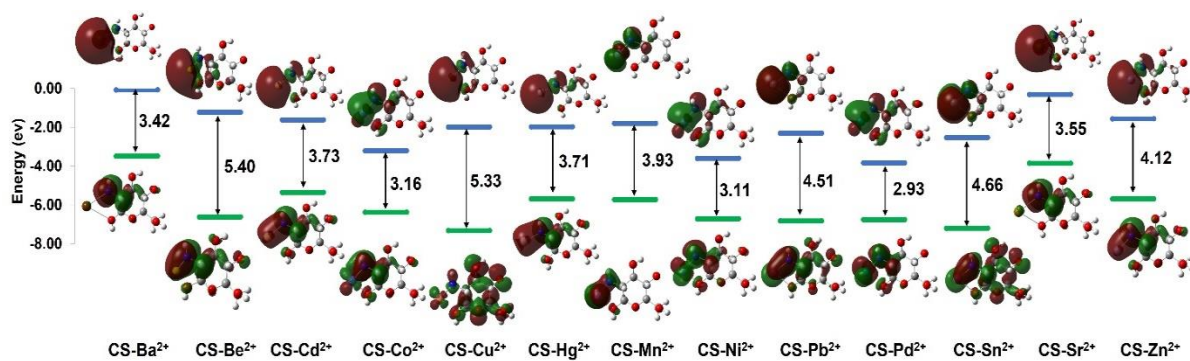
Figure 3 Energy diagram of HOMO and LUMO orbitals (in eV) of CS-divalent metal cation complexes.
