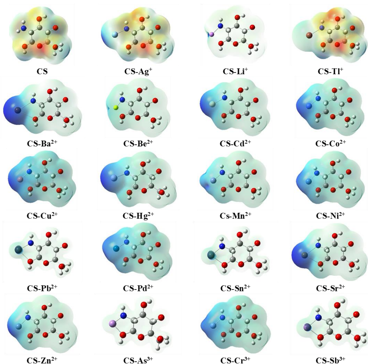
Figure 5 Molecular electrostatic potential (MEP) of CS and CS structure interacting with metals.
