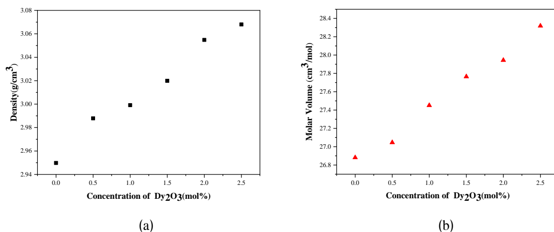
Figure 2 (a) Variation of density ( \rho ) and (b) molar volume ( V_M ) for the Dy 3+ doped ZnO-SrO-B 2 O 3 glass.
