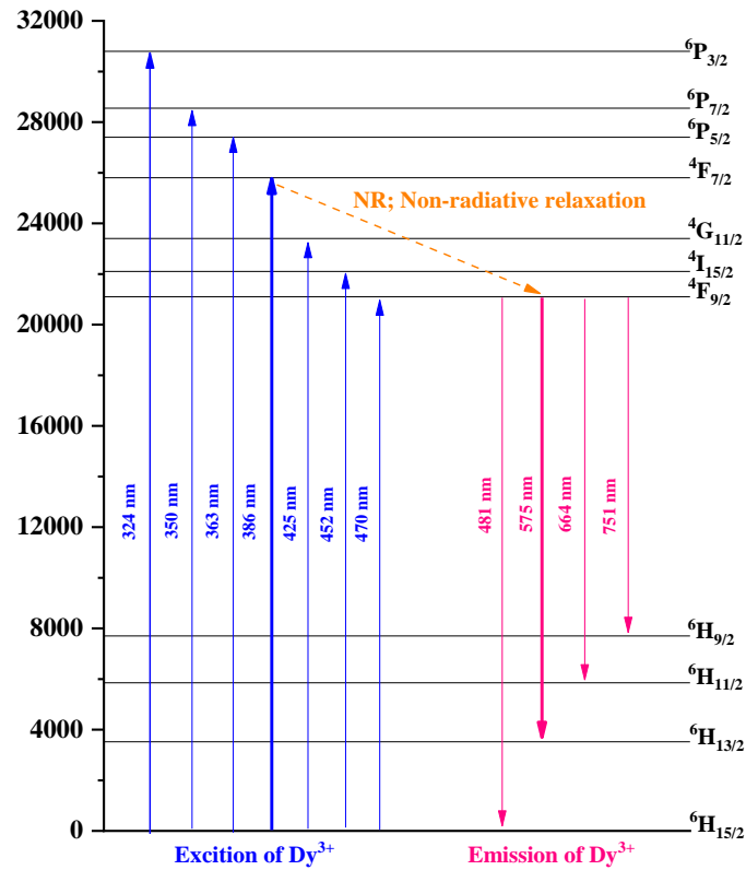
Figure 6 The Partial energy levels diagram of the \text{Dy}^{3+} ions in the \text{ZnO-SrO-B}_2\text{O}_3 glass.
