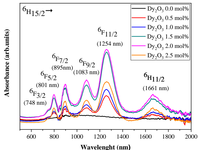
Figure 3 The absorption spectra of the ZnO-SrO-B 2 O 3 glass at different Dy 2 O 3 contents.
