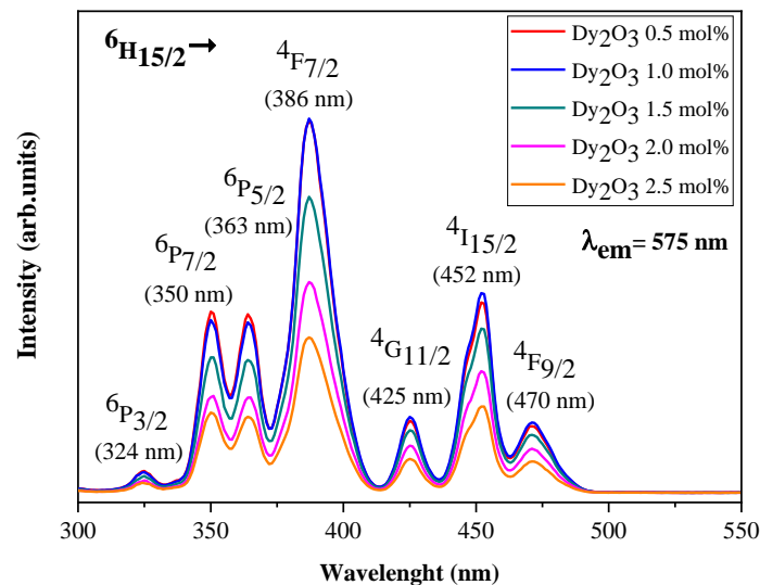
Figure 4 The excitation spectra of the ZnO-SrO-B 2 O 3 glass at different Dy 2 O 3 concentrations.
