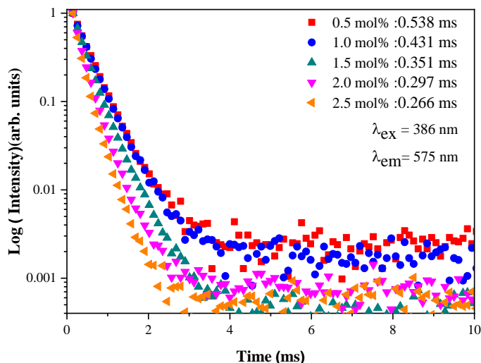
Figure 7 Luminescence decay profiles of the ^4F_{9/2} level of Dy^{3+} in ZnO-SrO-B_2O_3 glass at different Dy_2O_3 contents.
