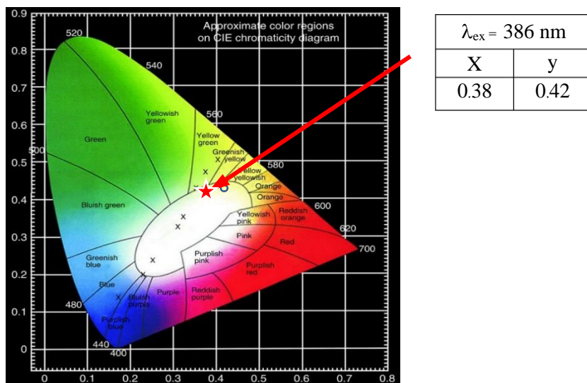
Figure 8 CIE chromaticity coordinates of ZnO-SrO-B_2O_3 glass at different Dy_2O_3 contents.
