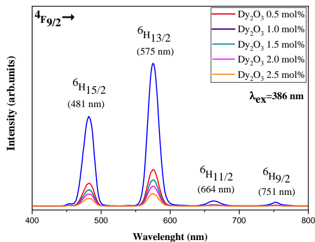
Figure 5 The emission spectra of the ZnO-SrO-B 2 O 3 glass at different Dy 2 O 3 contents.
